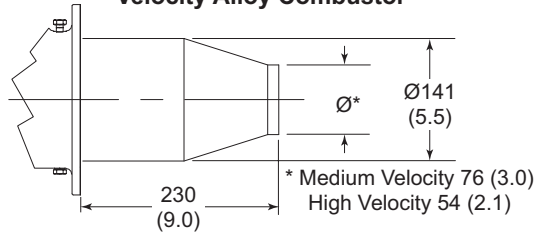
Medium & High Velocity Alloy Combustor
